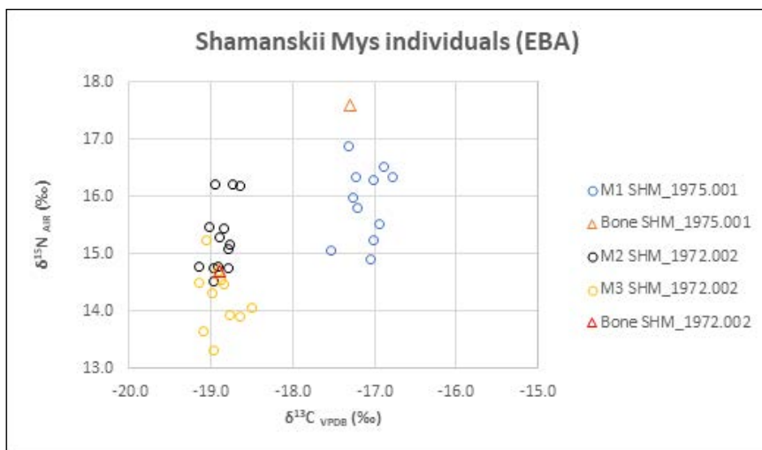
Figure 110. Stable isotope results for SHM_1975.001 and SHM_1972.002.
