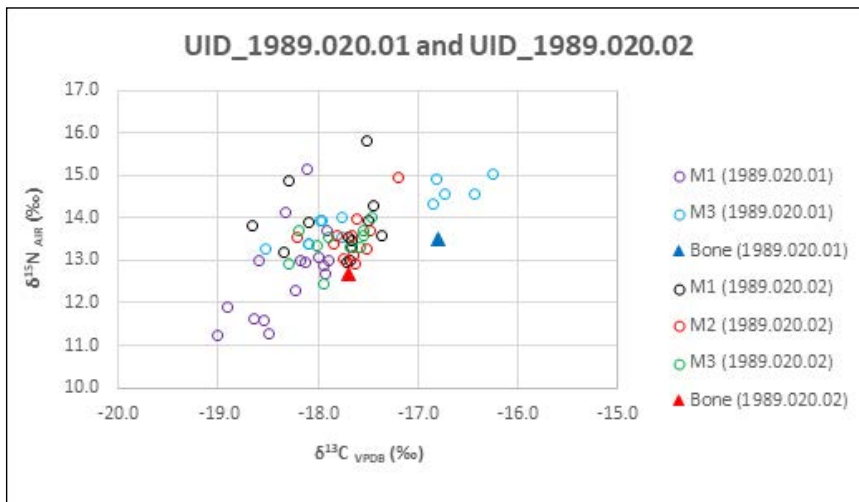
Figure 109. Stable isotope results for UID_1989.020.01 and UID_1989.020.02.
