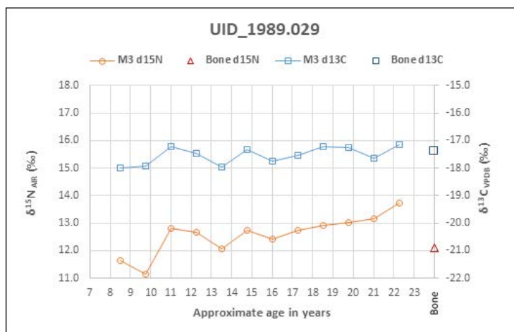
Figure 108. A continuous oscillation of both \delta^{13}\text{C} and \delta^{15}\text{N} in UID_1989.029 (M3).
