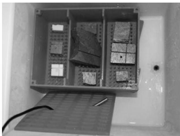
FIG. 10. THE INNER STRUCTURE OF THE FREEZE-THAW CHAMBER. BEFORE A FREEZING CYCLE STARTS, PURIFIED WATER DROPS FOR 30 MINUTES ONTO THE STONES, SIMULATING RAIN.
