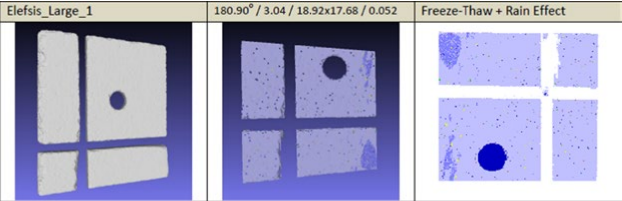
FIG. 20. DEPICTION OF GEOMETRY AND QEMSCAN REGISTRATION RESULTS FOR THE ELEFSIS LARGE 1 (EL1) MARBLE SLAB.
